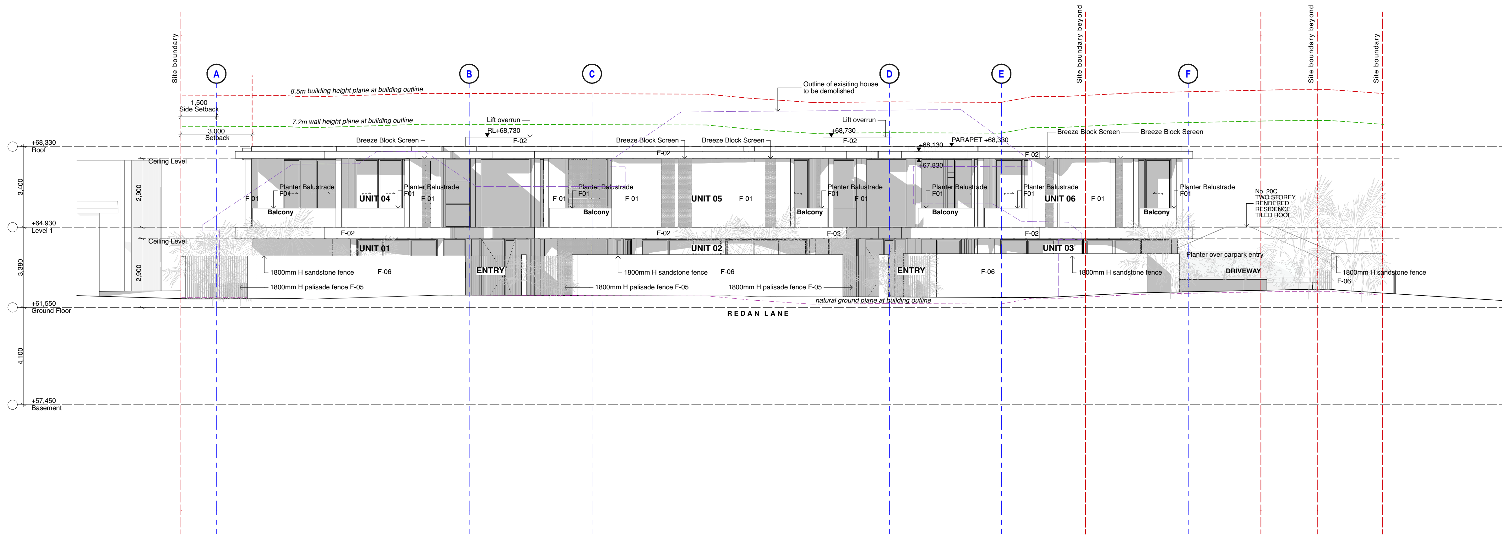
WEST ELEVATION
